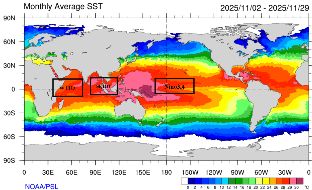
Gambar 1. Rata – rata Suhu Muka Laut Bulan November 2025
