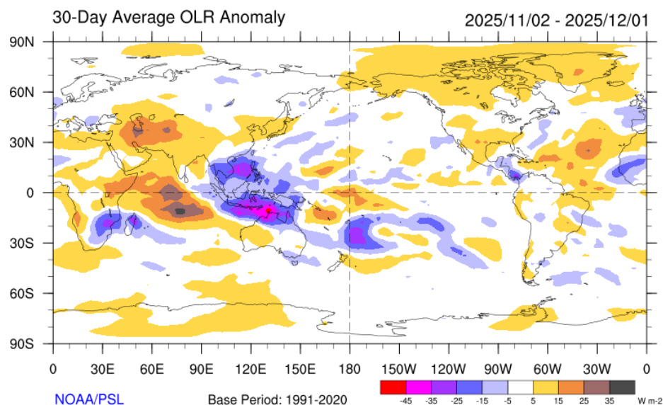
Gambar 5. OLR Anomali Bulan November 2025
