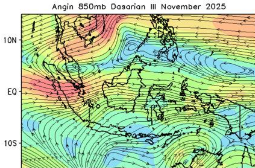
Gambar 8. Analisis Streamline Angin Dasarian III November 2025
