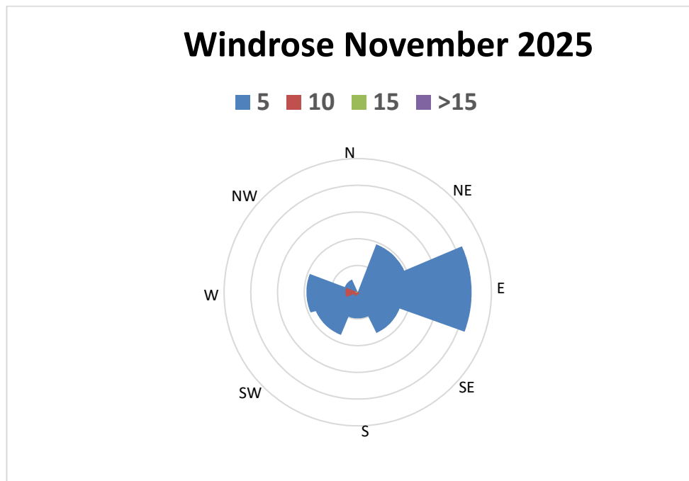
Gambar 11. Wind Rose Bulan November 2025
